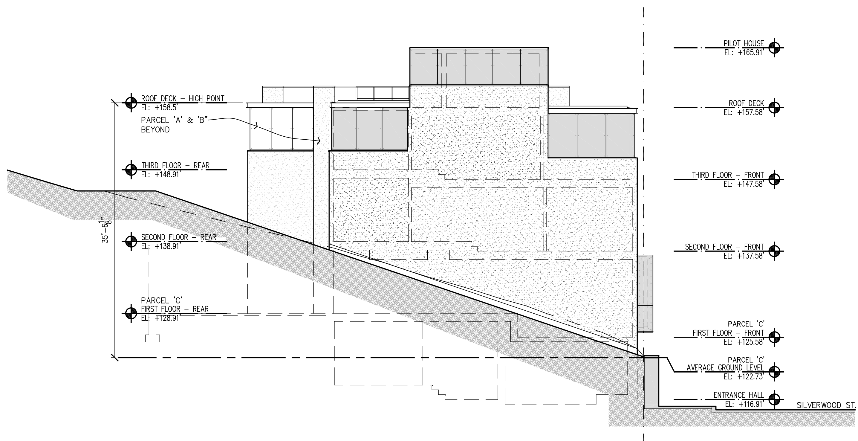
3 ZONING WEST ELEVATION - PARCEL 'C' 1/8" = 1'-0"
